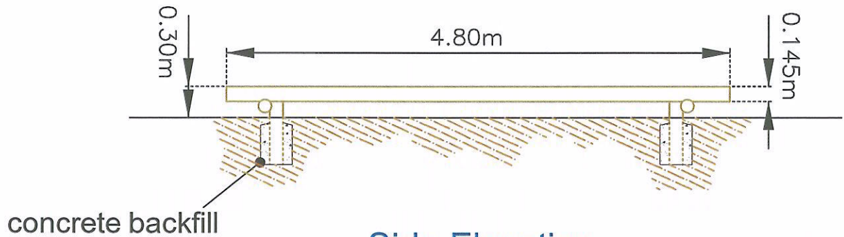
Side Elevation
