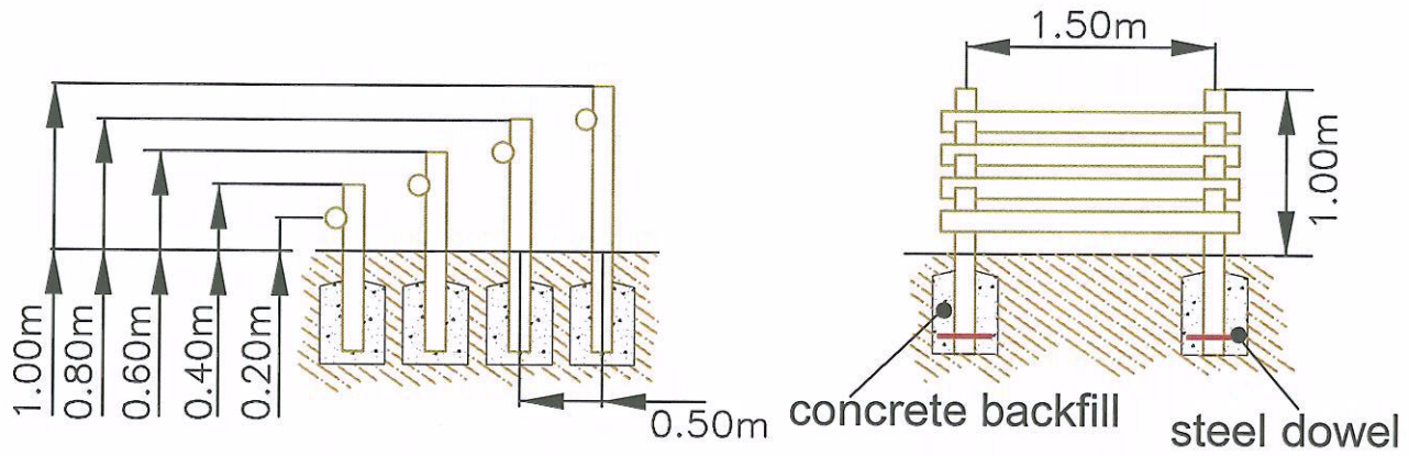
Side Elevation
