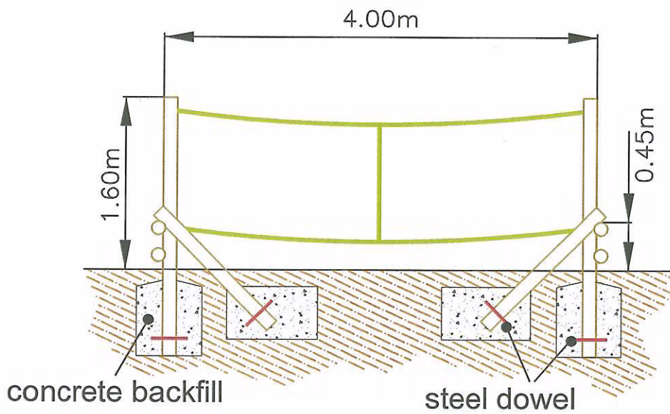
Side Elevation
