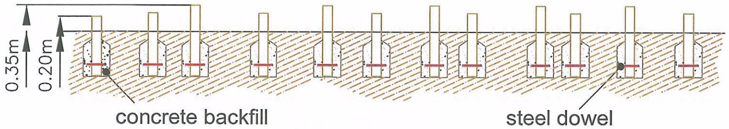
Side Elevation
