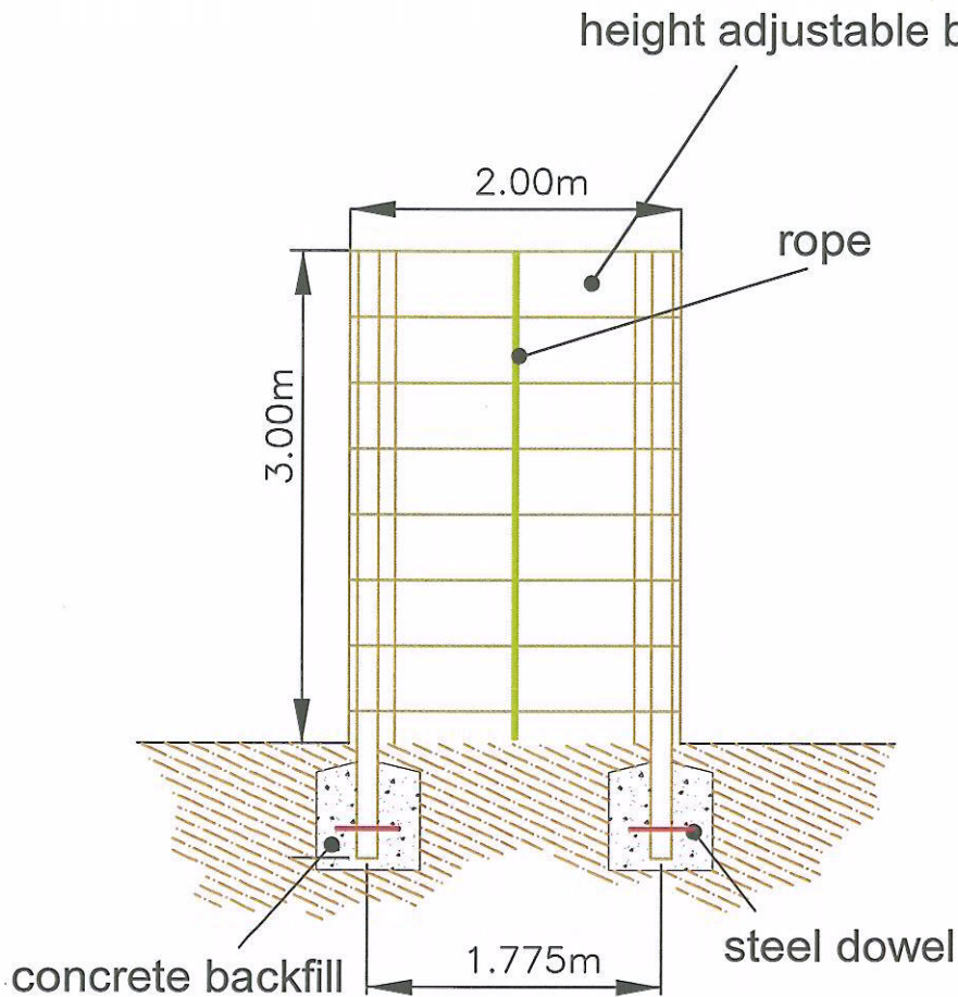
Side Elevation
