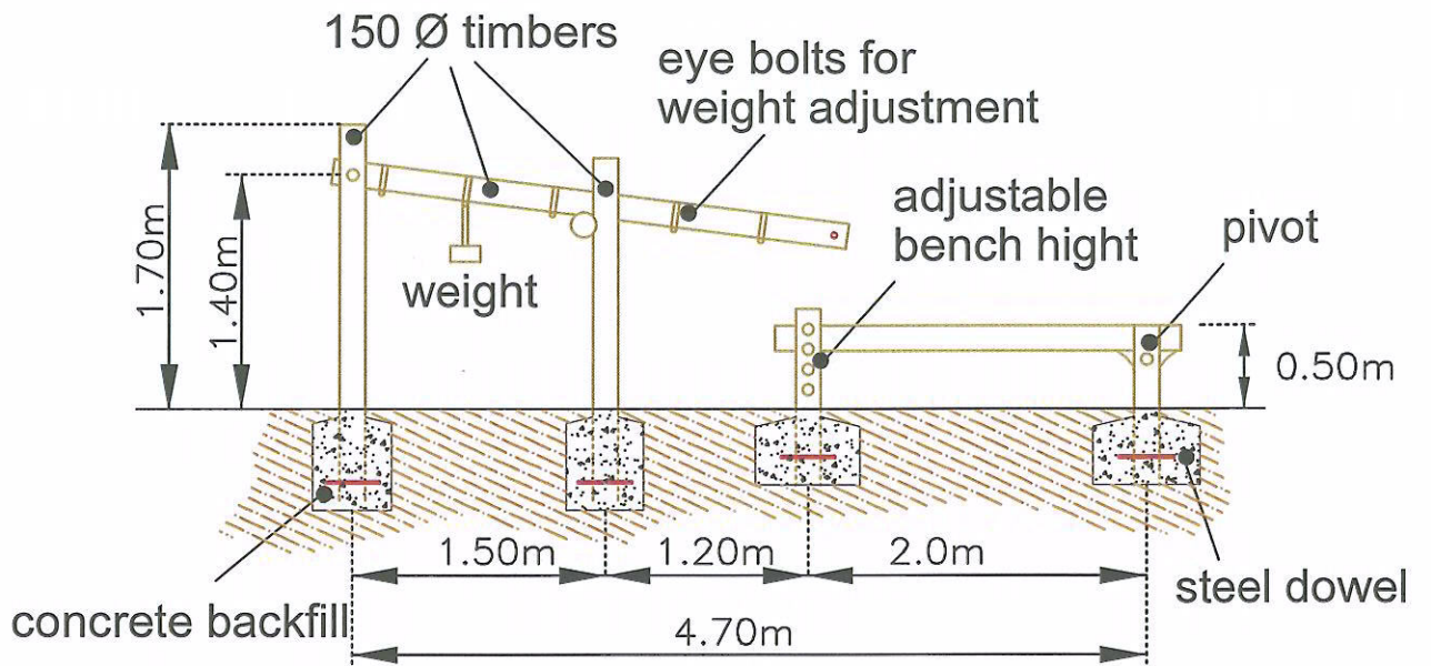
Front Elevation
